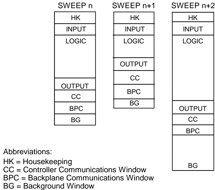
Figure 46: Typical Sweeps in Normal Sweep Mode
