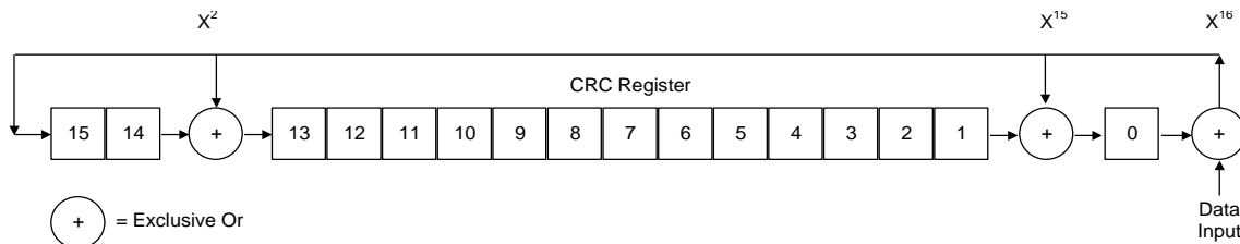
Figure 56: CRC Register Operation
